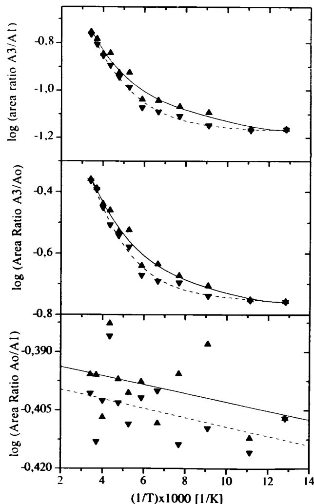
FIGURE 6 Plots of \log(\text{area ratios}) for conformer band ratios A_3/A_1 , A_3/A_0 , and A_0/A_1 versus 10^3/T in hydrated, unbuffered MbCO film with (0.30 g water)/(g MbCO). See Fig. 3 for details.
