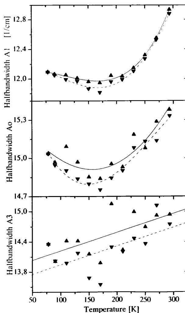
FIGURE 4 Temperature dependence of the half-bandwidths of the CO stretching bands of conformers A_0 , A_1 , and A_3 in hydrated unbuffered MbCO film with (0.30 g water)/(g MbCO). See Fig. 3 for details.
