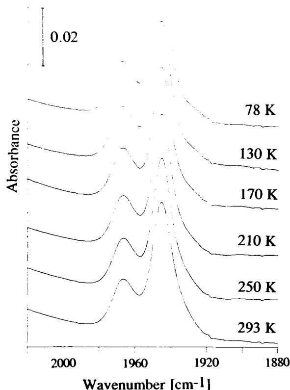
FIGURE 1 FTIR spectra of hydrated unbuffered MbCO film containing (0.30 g water)/(g MbCO) from 2020 to 1880 \text{cm}^{-1} , recorded on cooling from 293 K to 78 K at selected temperatures. Water vapor has been subtracted. The ordinate scale is for the spectrum recorded at 293 K. The other spectra are shown at similar size and are shifted vertically for clarity.
