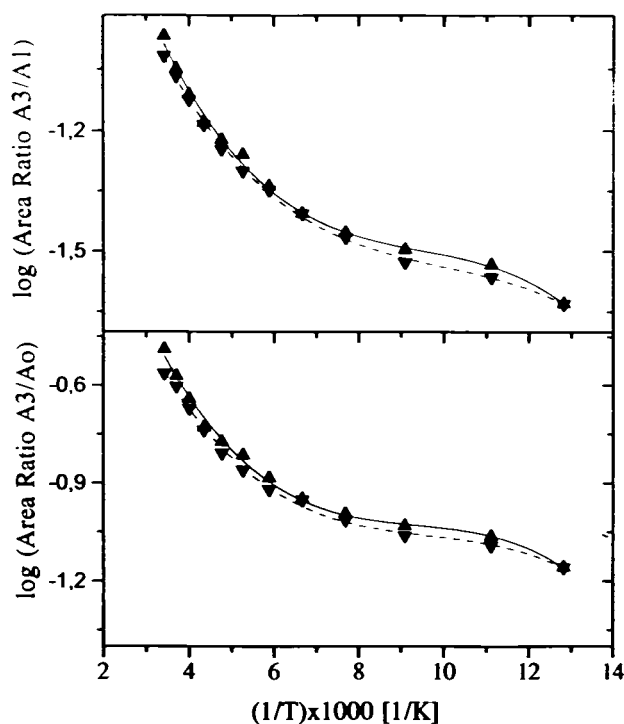
FIGURE 9 Plots of \log(\text{area ratio } A_3/A_1) and \log(\text{area ratio } A_3/A_0) versus 10^3/T in hydrated, buffer-containing MbCO film with (0.32 \text{ g water})/(\text{g MbCO}) . See Fig. 3 for details.
